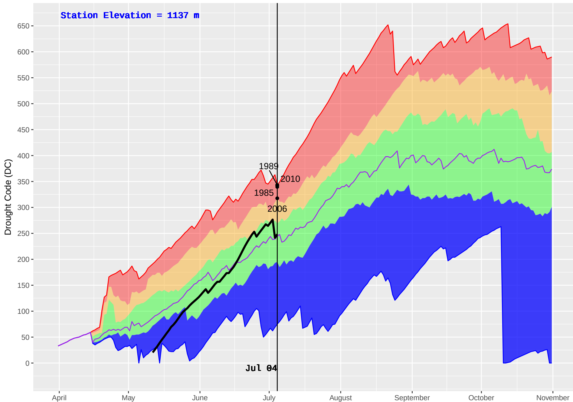
KLUSKUS (166) : Historical (1982–2016) and Current (2018) Noon Drought Code (DC)
